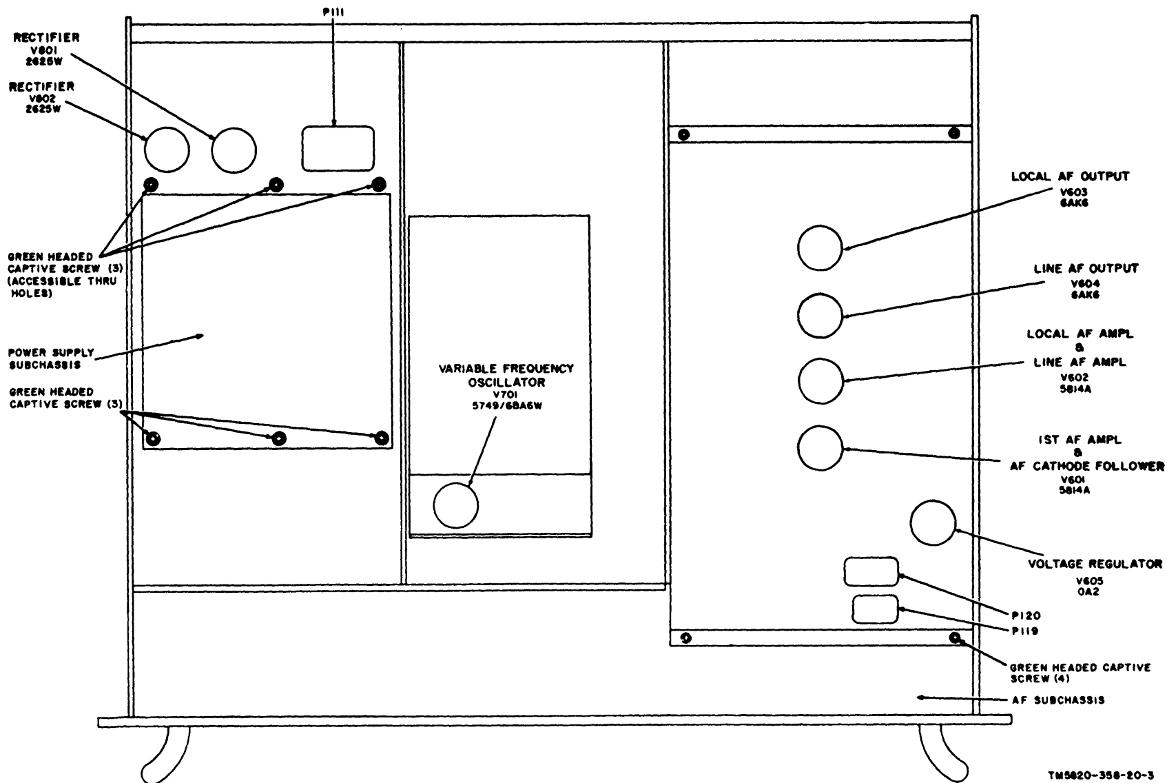
Figure 3. Radio Receiver R-390A/URR, bottom deck, tube, and subchassis location.
