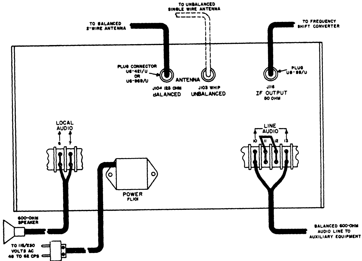
Figure 5. Cording diagram.
