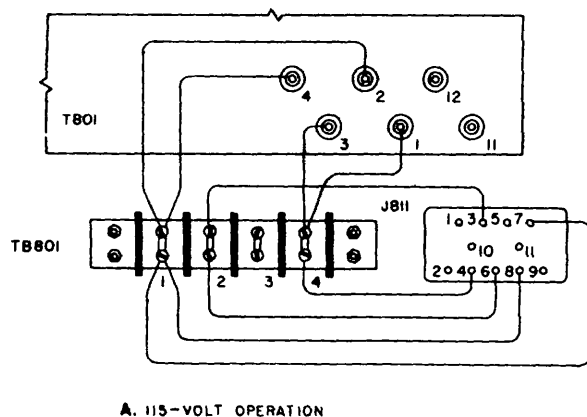
Figure 6. Connection for 115-volt or 230-volt operation.
