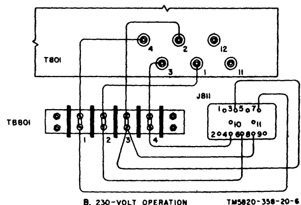
Figure 6. Connection for 115-volt or 230-volt operation.
